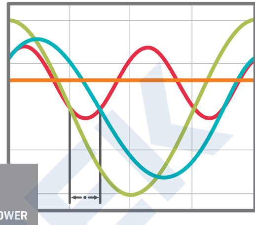
Figure 3: Instantaneous and average power calculated from ac voltage and current with a lagging power factor of 0.71
